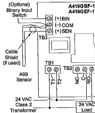
Figure 9: Wiring the 24 VAC A419 Control
