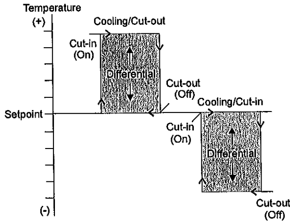
Figure 7: Cooling Modes
