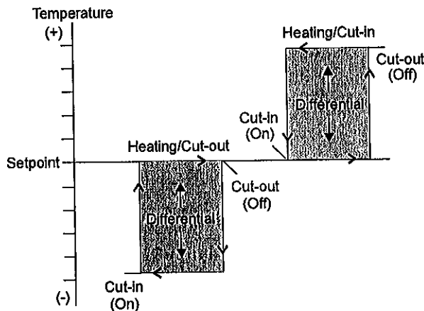
Figure 8: Heating Modes
